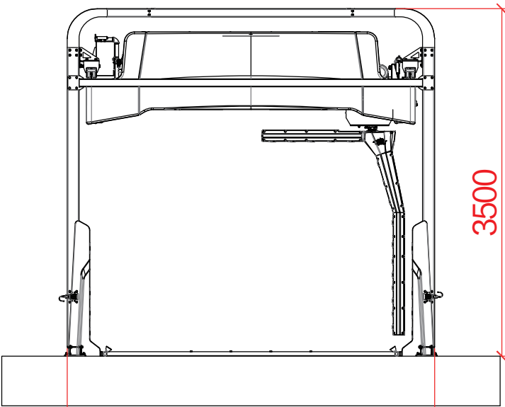
EQUIPMENT FRONT VIEW
