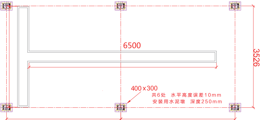
INSTALLATION FLOOR VERTICAL VIEW
