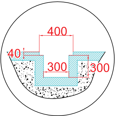
WATERWAY SECTIONAL VIEW
